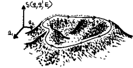
Figure 34.2: A romanticized sketch of S_\rho(E) = S(q, q, E) = \oint p(q, E) dq landscape orbit. Unstable periodic orbits traverse isolated ridges and saddles of the mountainous landscape of the action S(q_\parallel, q_\perp, E) . Along a periodic orbit S_\rho(E) is constant; in the transverse directions it generically changes quadratically.
