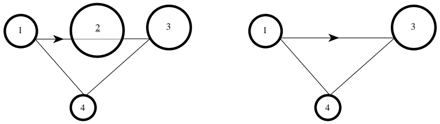
Figure 36.6: (a) The ghost itinerary (1, 2 , 3, 4). (b) The parent itinerary (1, 3, 4 ).
