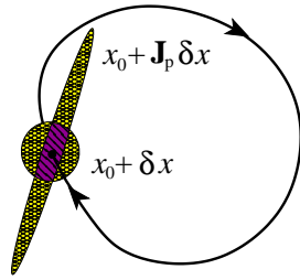
Figure 5.1: For a prime cycle p , Floquet matrix J_p returns an infinitesimal spherical neighborhood of x_0 \in M_p stretched into an ellipsoid, with overlap ratio along the eigdirection \mathbf{e}^{(j)} of J_p(x) given by the Floquet multiplier |\Lambda_{p,j}| . These ratios are invariant under smooth nonlinear reparametrizations of state space coordinates, and are intrinsic property of cycle p .
