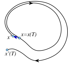
Figure 5.2: An unstable periodic orbit repels every neighboring trajectory x'(t) , except those on its center and unstable manifolds.
