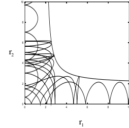
Figure 30.1: A typical collinear helium trajectory in the r_1 - r_2 plane; the trajectory enters along the r_1 axis and escapes to infinity along the r_2 axis.
