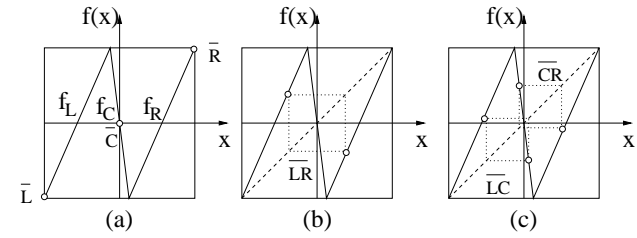
Figure 9.2: The D_1 -equivariant bimodal sawtooth map of figure 9.1 has three types of periodic orbits: (a) D_1 -fixed fixed point C , asymmetric fixed points pair \{\bar{L}, \bar{R}\} . (b) D_1 -symmetric (setwise invariant) 2-cycle \bar{L}\bar{R} . (c) Asymmetric 2-cycles pair \{\bar{L}\bar{C}, \bar{C}\bar{R}\} . (continued in figure 9.8) (Y. Lan)
