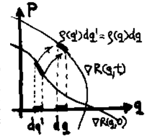
Figure 33.2: Density evolution of an initial surface (q', p' = \partial_{q'} R(q', 0)) into (q(t), p(t)) surface time t later, sketched in 1 dimension. While the number of trajectories and the phase space Liouville volume are conserved, the density of trajectories projected on the q coordinate varies; trajectories which started in dq' at time zero end up in the interval dq .
