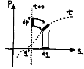
Figure 33.4: Evolution of the semiclassical propagator. The configuration which corresponds to the initial conditions of the propagator is a Lagrangian manifold q = q' , that is, a plane parallel to the p axis. The hypothetical particles are thus initially all placed at q' but take on all possible momenta p' . The Jacobian matrix C (33.29) relates an initial volume element in momentum space dp' to a final configuration space volume dq .
