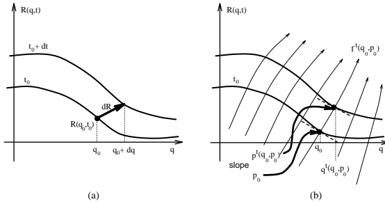
Figure 33.1: (a) A phase R(q,t) plotted as a function of the position q for two infinitesimally close times. (b) The phase R(q,t) transported by a swarm of “particles”; The Hamilton’s equations (33.10) construct R(q,t) by transporting q_0 \rightarrow q(t) and the slope of R(q_0, t_0) , that is p_0 \rightarrow p(t) .
