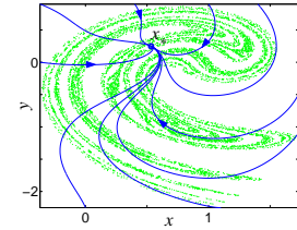
Figure 29.3: Typical trajectories of the vector field (29.9) for the stabilization of a hyperbolic fixed point of the Ikeda map (29.11) located at (x, y) \approx (0.53275, 0.24689) . The circle indicates the position of the fixed point. Note that the basin of attraction of this fixed point is large, larger than the entire Ikeda attractor.
