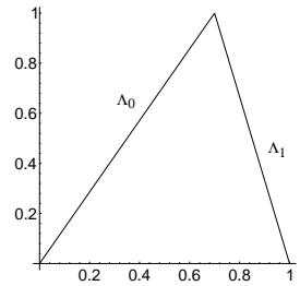
Figure 16.3: A piecewise-linear skew 'full tent map' (16.11) ( \Lambda_0 = 4/3 , \Lambda_1 = -4 ).
