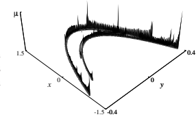
Figure 16.5: Natural measure (16.19) for the Hénon map (3.19) strange attractor at parameter values (a, b) = (1.4, 0.3) . See figure 3.9 for a sketch of the attractor without the natural measure binning. (Courtesy of J.-P. Eckmann)
