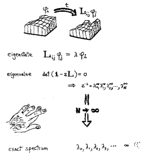
Figure 16.4: State space discretization approach to computing averages.
