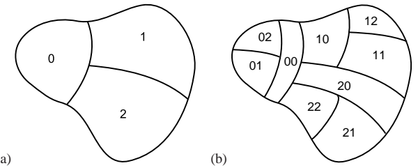
Figure 16.1: (a) First level of partitioning: A coarse partition of M into regions M_0 , M_1 , and M_2 . (b) n = 2 level of partitioning: A refinement of the above partition, with each region M_i subdivided into M_{i0} , M_{i1} , and M_{i2} .
