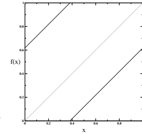
Figure 27.1: Unperturbed circle map ( k = 0 in (27.1)) with golden mean rotation number.
