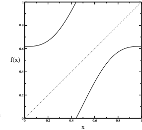
Figure 27.3: Critical circle map ( k = 1 in (27.1)) with golden mean bare rotation number.
