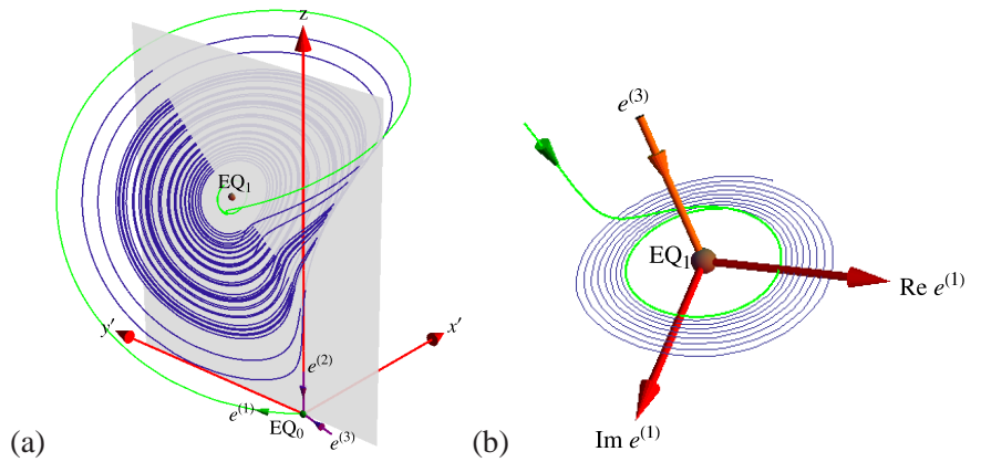
Figure 9.4: (a) Lorenz attractor plotted in [x', y', z] , the doubled-polar angle coordinates (9.21), with points related by \pi -rotation in the [x, y] plane identified. Stable eigenvectors of EQ_0 : \mathbf{e}^{(3)} and \mathbf{e}^{(2)} , along the z axis (9.20). Unstable manifold orbit W^u(EQ_0) (green) is a continuation of the unstable \mathbf{e}^{(1)} of EQ_0 . (b) Blow-up of the region near EQ_1 : The unstable eigenplane of EQ_1 defined by \text{Re } \mathbf{e}^{(2)} and \text{Im } \mathbf{e}^{(2)} , the stable eigenvector \mathbf{e}^{(3)} . The descent of the EQ_0 unstable manifold (green) defines the innermost edge of the strange attractor. As it is clear from (a), it also defines its outermost edge. (E. Siminos)
