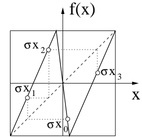
Figure 9.1: The bimodal Ulam sawtooth map with the D_1 symmetry f(-x) = -f(x) . If the trajectory x_0 \rightarrow x_1 \rightarrow x_2 \rightarrow \dots is a solution, so is its reflection \sigma x_0 \rightarrow \sigma x_1 \rightarrow \sigma x_2 \rightarrow \dots . (continued in figure 9.2)
