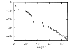
Figure 15.2: The logarithm \ln|z_0^{(n)} - z_0| of the difference between the leading zero of the n -th polynomial approximation to topological zeta function and our best estimate (15.33), as a function of order of the polynomial n (the topological zeta function evaluated for the closest value of A to A = 3.8 for which the quadratic map has a stable cycle of period n ). (from K.T. Hansen [12.19])
