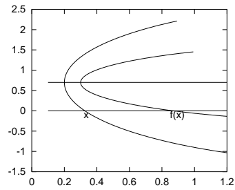
Figure C.1: Illustration of the optimal Poincaré surface. The original surface y = 0 yields a large distance x - f(x) for the Newton iteration. A much better choice is y = 0.7 .
